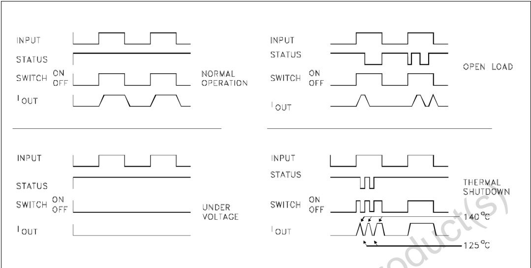
Figure 4. Waveforms
